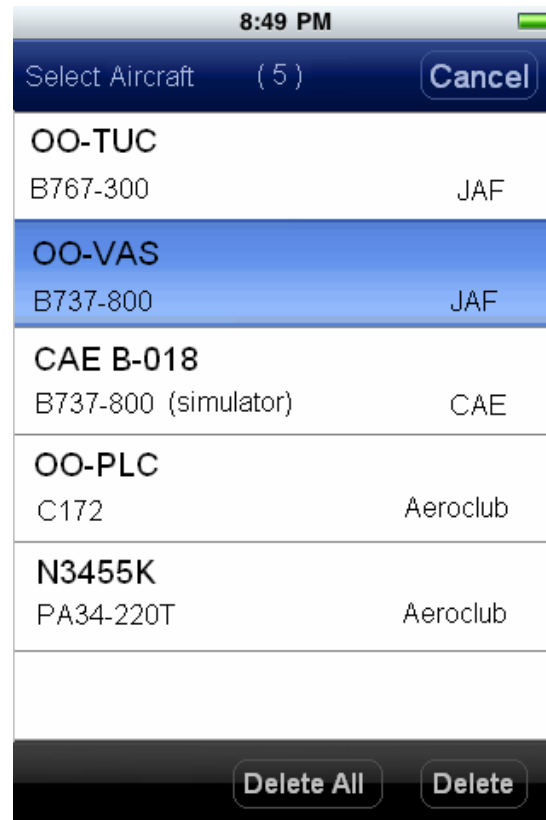
Aircraft List
